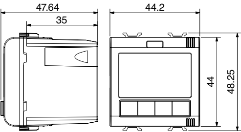
GW 1x 709 Termostato connesso
